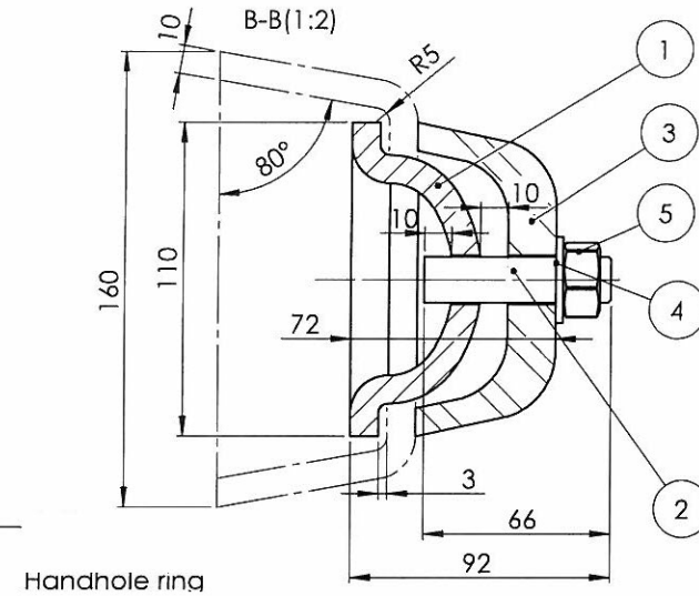
Handhole ring
