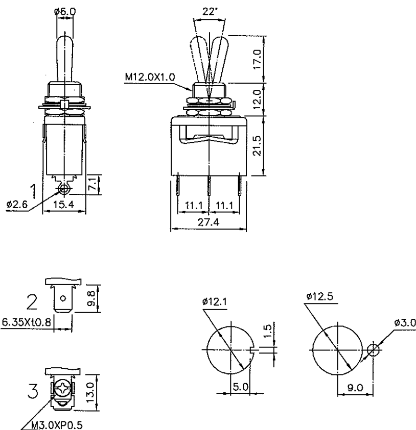
PANEL LAYOUT
