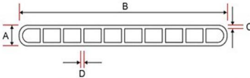
Aluminium Micro MultiPort Extruded Profile Tube
