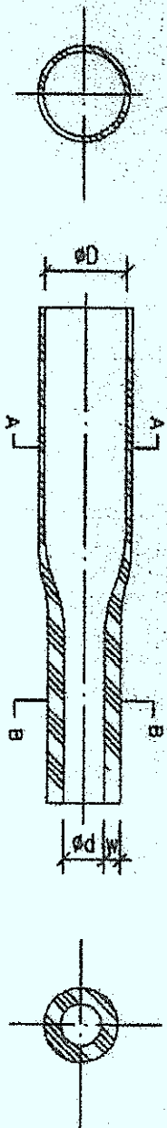
A--A(As Supplied)
